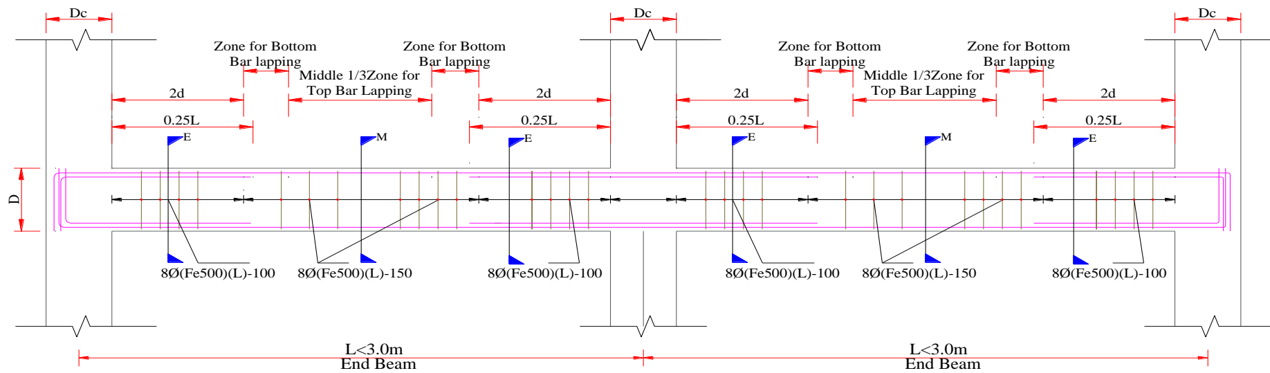
TYPICAL L-SECTION OF FLOOR BEAM (ALONG BEAM 1)
