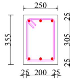
Typical Beam Section P-P
