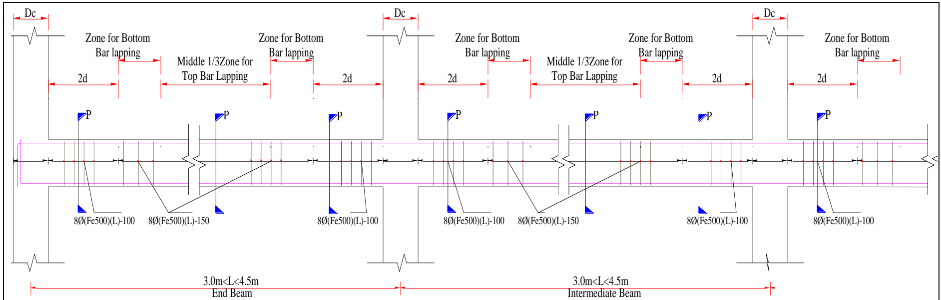
TYPICAL L-SECTION OF PLINTH BEAM (ALONG BEAM 2)
