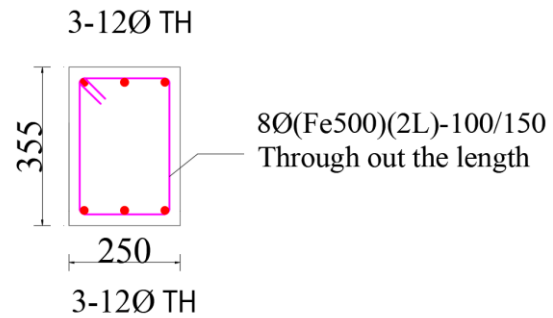
Plinth Tie Beam Section P-P
