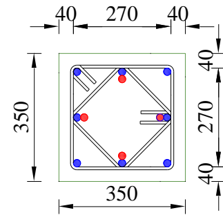
● - Curtailed Bar ● - Spliced Bar Typical Column (350x350mm) Section At Splicing/Lapping Zone
