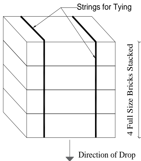
FIGURE 3-1 DROPPING WEIGHT METHOD FOR APPROXIMATION OF SBC
