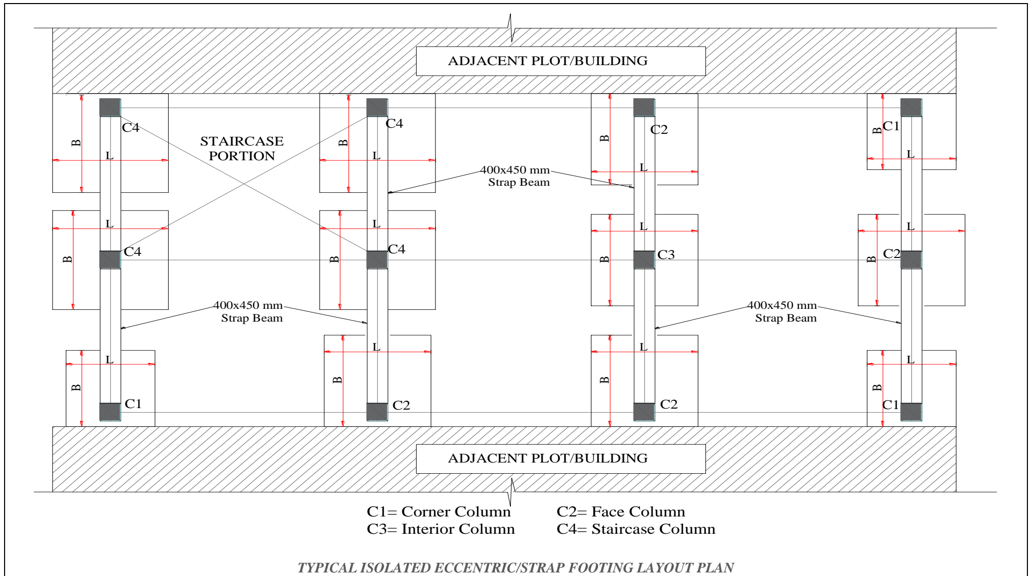
FIGURE 9-2 TYPICAL ECCENTRIC FOOTING DETAIL OF THREE STOREY BUILDING
