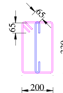
Size of Stirrups of dia 8mm
