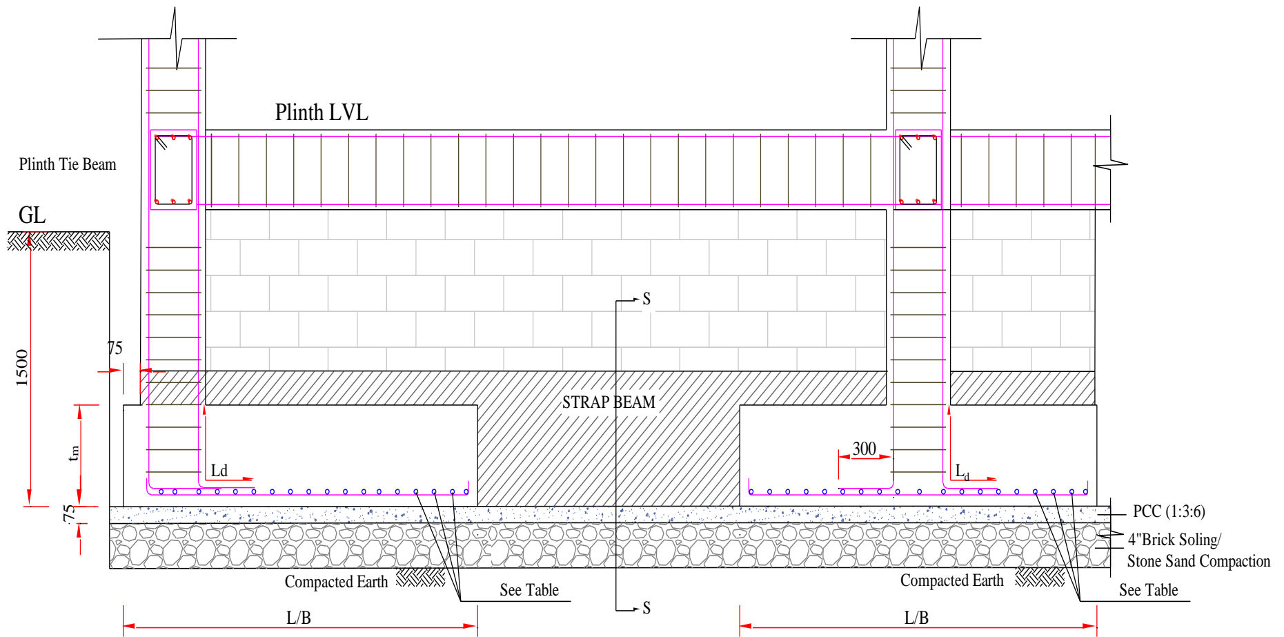
TYPICAL ISOLATED ECCENTRIC/STRAP FOOTING SECTION
