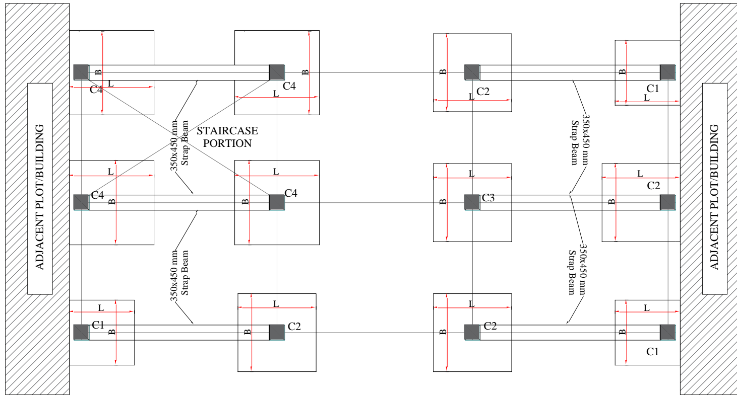
FIGURE 8-3 (B) TYPICAL ECCENTRIC FOOTING DETAIL
