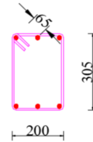
Size of Stirrups of dia 8mm
