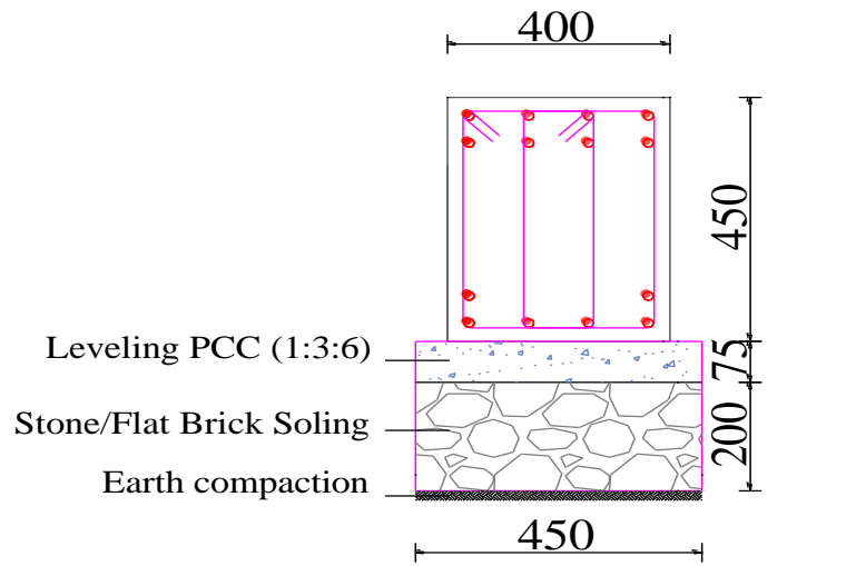
STRAP BEAM (SECTION S-S)
