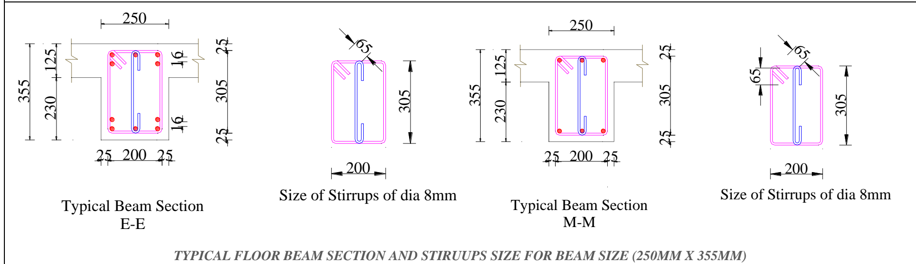
TYPICAL FLOOR BEAM SECTION AND STIRRUPS SIZE FOR BEAM SIZE (250MM X 355MM)
