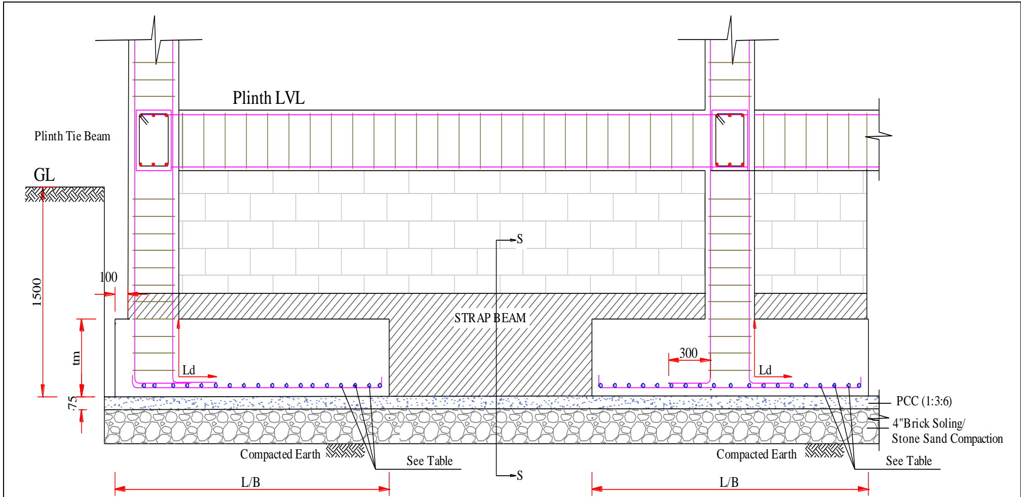
TYPICAL ISOLATED ECCENTRIC/STRAP FOOTING SECTION
