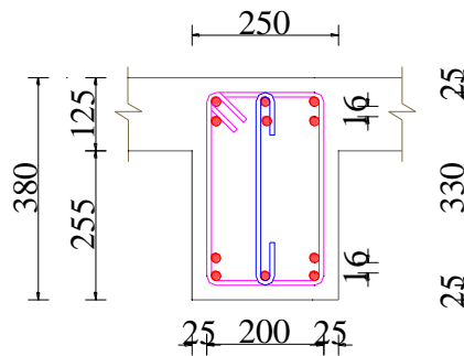
Typical Beam Section E-E
