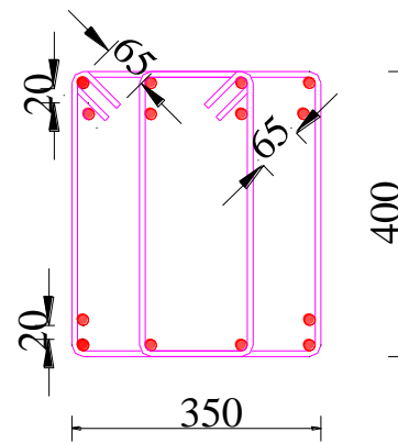
SIZE OF STIRRUPS OF DIA 8MM
