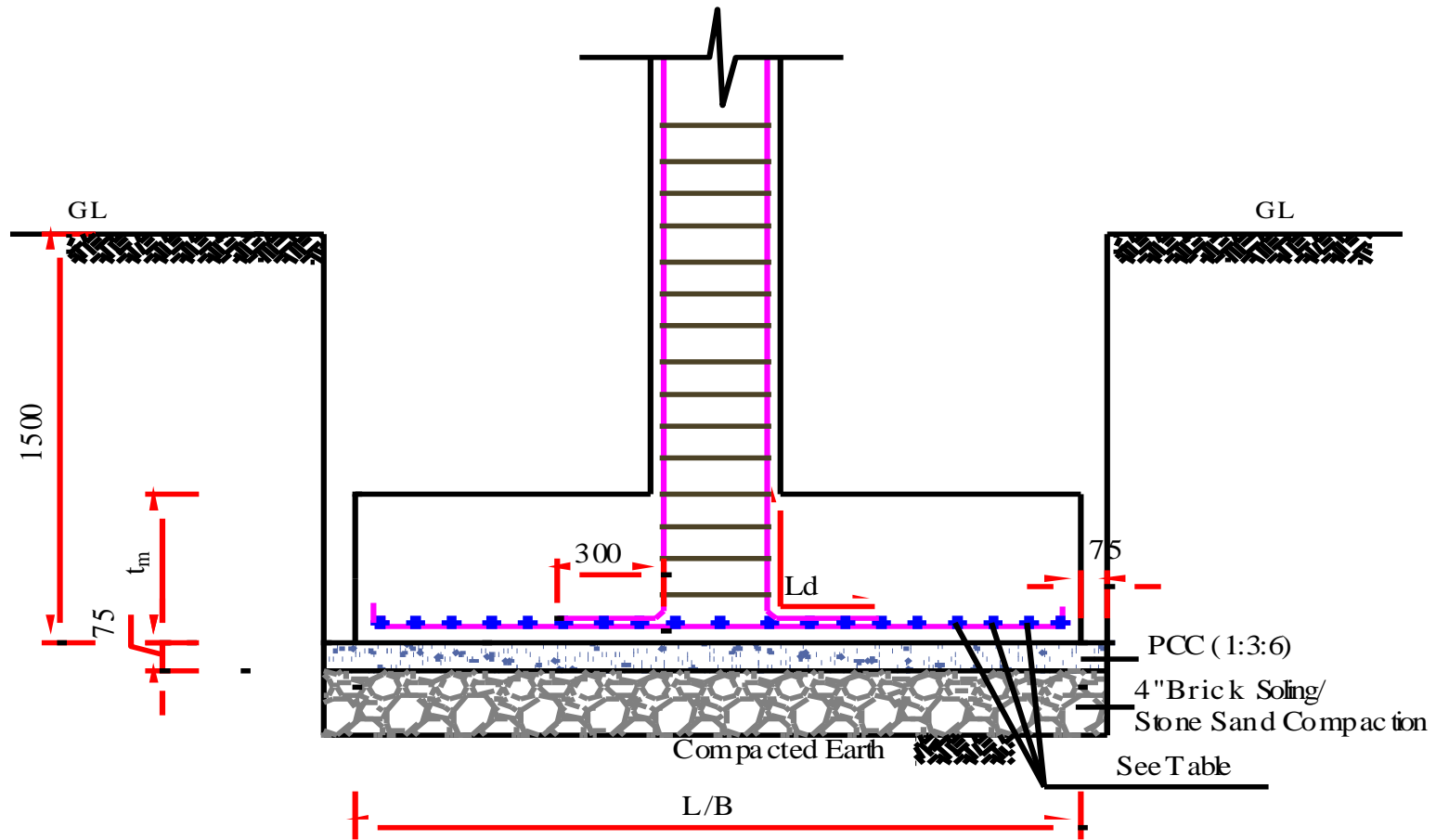
TYPICAL ISOLATED FOOTING SECTION COVER FOR SIDE FACE = 75 MM; COVER FOR BOTTOM FACE = 50 MM
