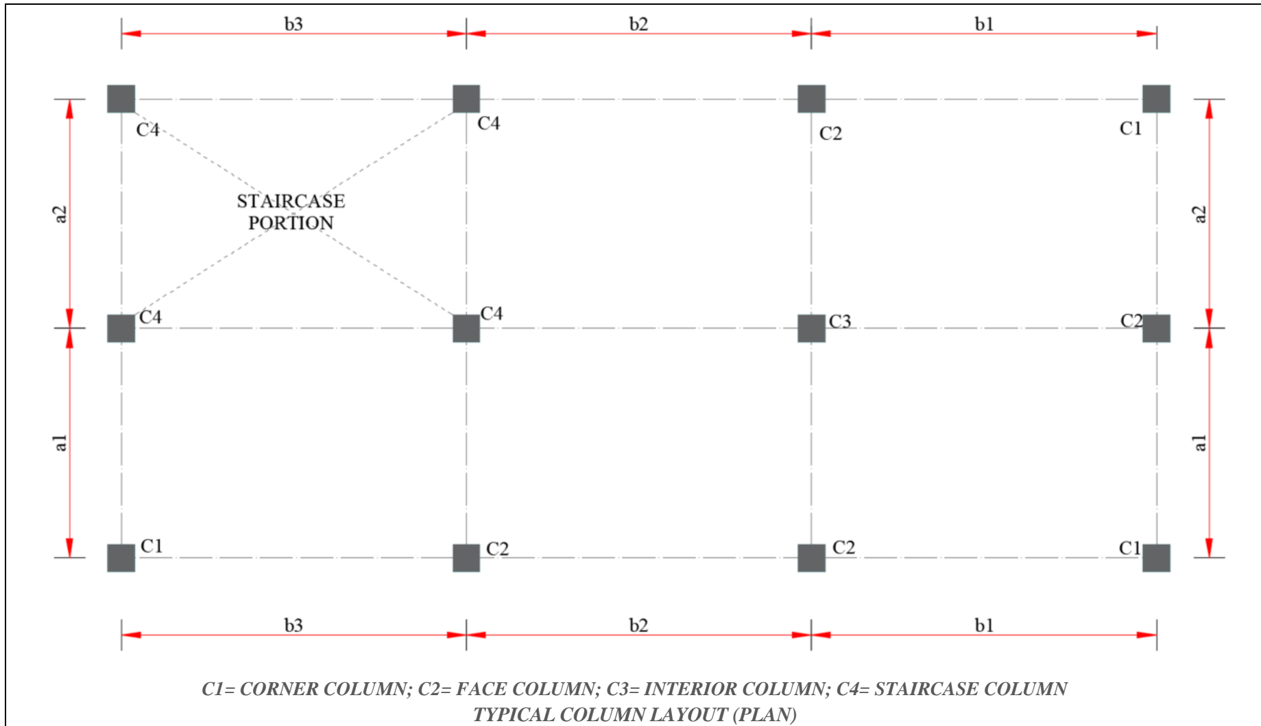
FIGURE 9-4 TYPICAL COLUMN DETAIL FOR THREE STOREY BUILDING
