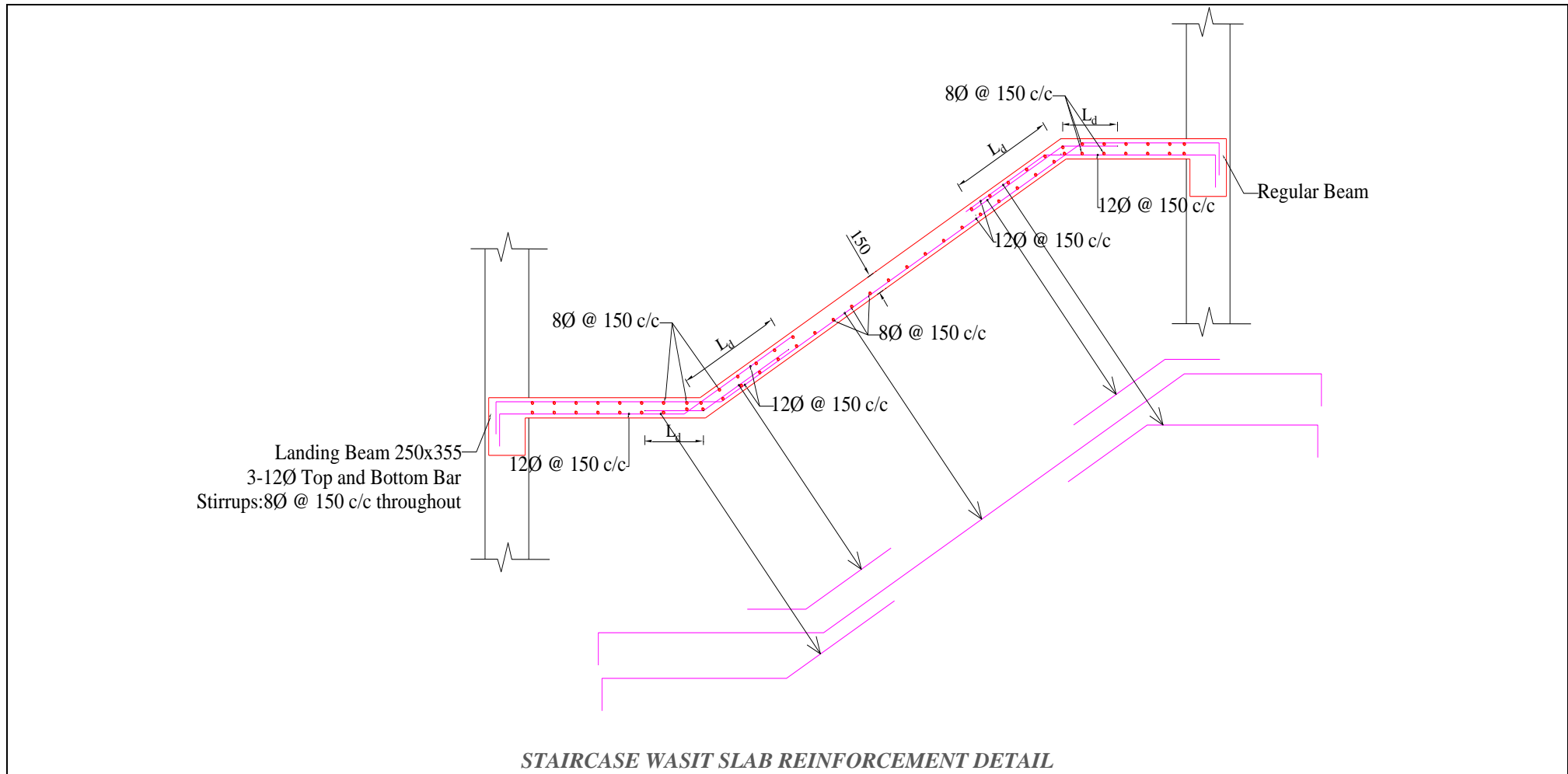
FIGURE 10-5 STAIRCASE DETAIL (OPTION I- WITH RCC STEPS) & (OPTION II- WITH MASORNY STEPS)
