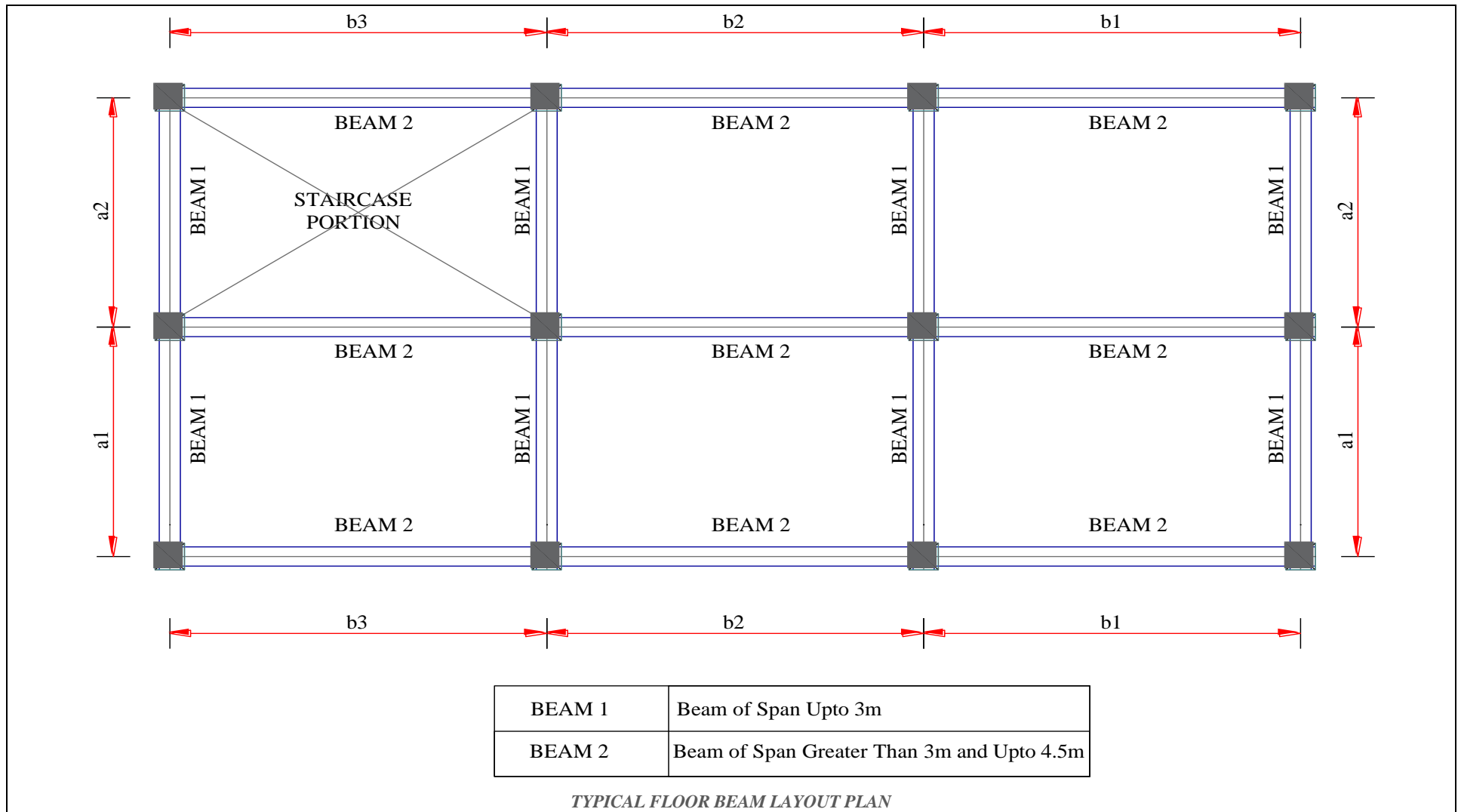
FIGURE 9-5 TYPICAL FLOOR BEAM DETAIL OF THREE STOREY BUILDING
