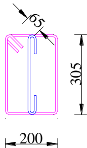
Size of Stirrups of dia 8mm
