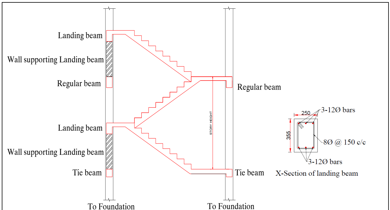
FIGURE 10-4 STAIRCASE LANDING BEAM ARRANGEMENT AND REINFORCEMENT DETAIL
