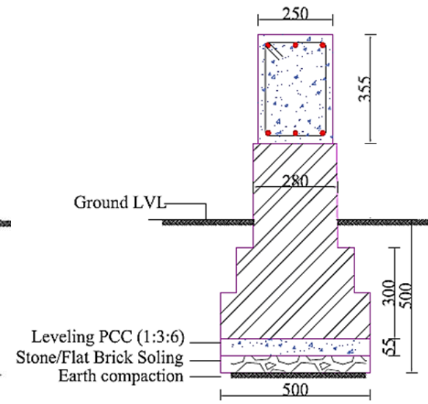
BRICK MASONRY TOE WALL
