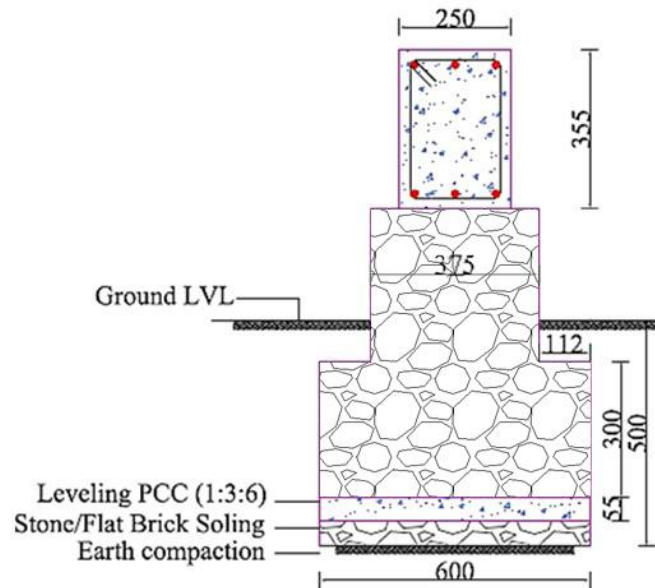
STONE MASONRY TOE WALL
