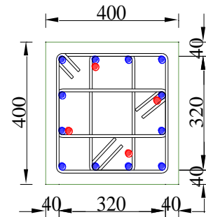
● - Curtailed Bar ● - Spliced Bar Typical Column (400x400mm) Section At Splicing/Lapping Zone
