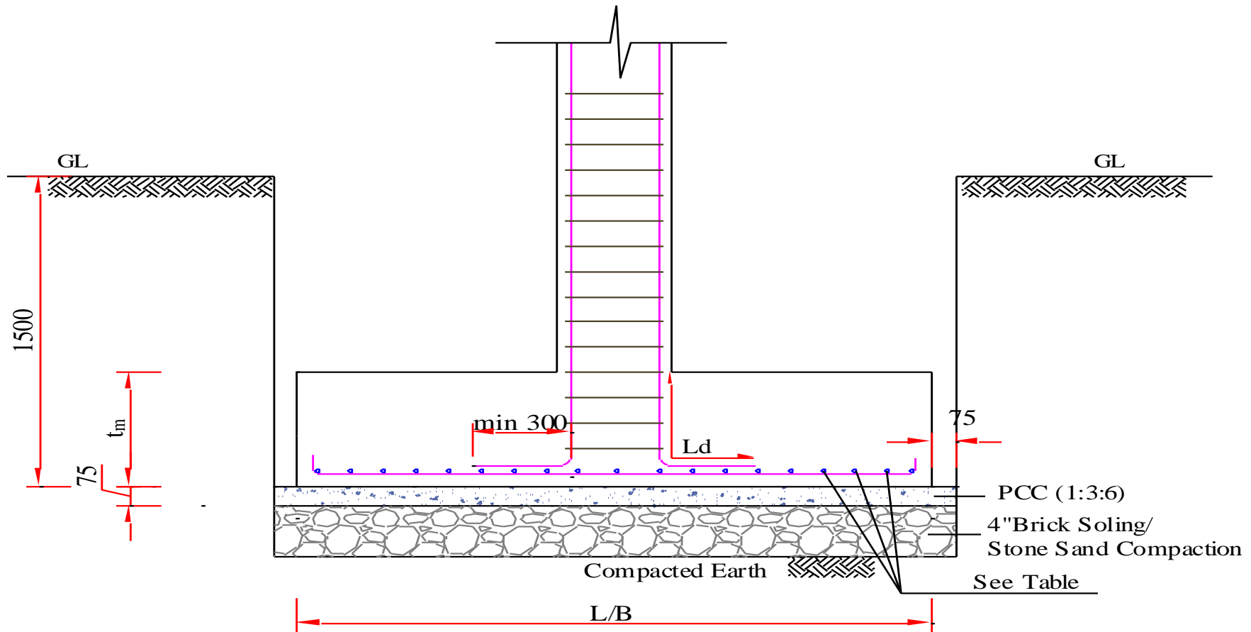
TYPICAL ISOLATED FOOTING SECTION COVER FOR SIDE FACE = 75 MM; COVER FOR BOTTOM FACE = 50 MM
