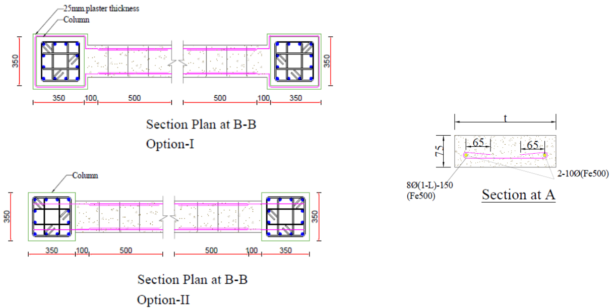
FIGURE 11-1 REINFORCEMENT DETAILS FOR SOLID WALL
