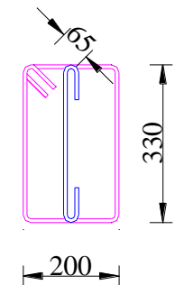
Size of Stirrups of dia 8mm
